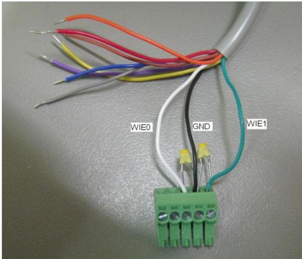
Picture 1. Adding capacitors to WIE-lines
