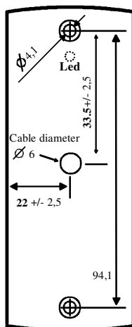
Access housing
